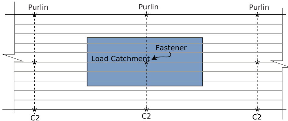
Symmetrical fastener pattern
