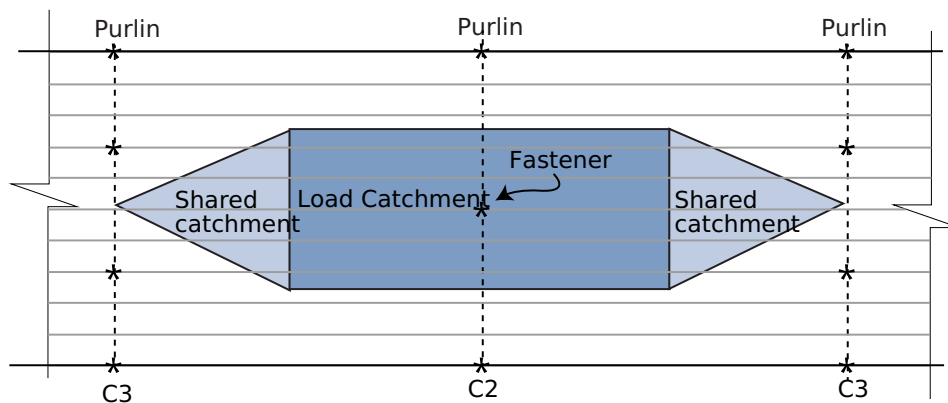
Asymmetrical fastener pattern
