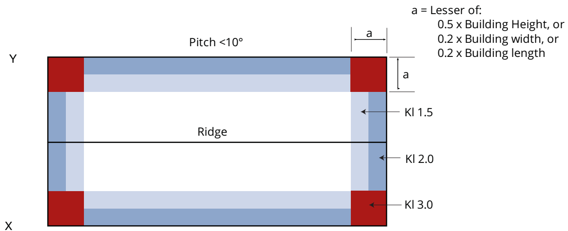
Local Pressure (KI) factors as per AS/NZS 1170:2011
